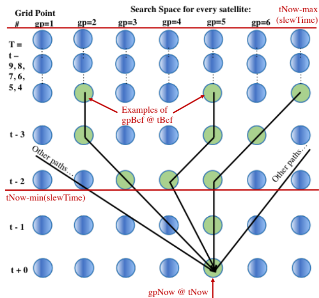
Figure 4—State space searched by the scheduler to compute the optimum path ending at [gpNow, tNow] , with no FOR overlaps
