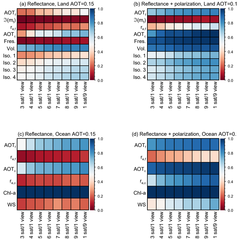
Figure 9. Diagonal values for the mean averaging kernel matrices, \mathbf{A} , for land scenes (a, b), ocean scenes (c, d) using observations of reflectance only (a, c) and DoLP with reflectance (b, d). These values roughly represent what fraction of a retrieved parameter is due to the observations and not a priori values. Results are shown for each satellite configuration (abscissa), while the ordinate axis has the results for each parameter described in Table 2. For the land scene, these parameters are, from the top, fine-size-mode AOT, imaginary component of the refractive index of the fine size mode, effective radius for the fine size mode, coarse-size-mode AOT, fresnel (polarized) surface reflectance coefficient, volumetric (BRDF shape) surface reflectance coefficient and isotropic reflectance coefficients for each band, at 410, 555, 865 and 2250 nm. For the ocean scene, these parameters are, from the top: fine-size-mode AOT, effective radius for the fine size mode, coarse-size-mode AOT, effective radius for the coarse size mode, ocean body Chl a content and ocean surface wind speed. The sum of each column is the DFS for each instrument configuration as shown in Fig. 6. This figure therefore displays how those DFS values are partitioned among the retrieval parameters.
