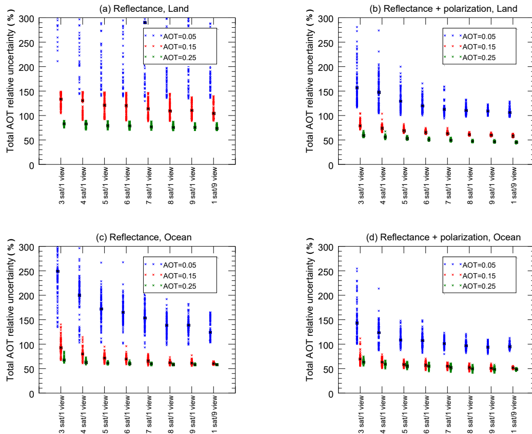
Figure 7. Aerosol optical thickness (AOT) relative uncertainty at 555 nm is plotted for continental aerosols over land ( a, b ), maritime aerosols over ocean ( c, d ) for instruments using reflectance alone ( a, c ) and reflectance plus DoLP ( b, d ). The simulated aerosol load is indicated by color and position, where AOT (555 nm) equal to 0.05 is blue (left), AOT (555 nm) equal to 0.15 is red (center) and AOT (555 nm) equal to 0.25 is green (right). The number of single-view satellites is indicated along the abscissa, with the exception of the nine-view “multi-angle” single instrument at the far right. The ordinate axis is the relative uncertainty of the total (fine- and coarse-size-mode) AOT.
